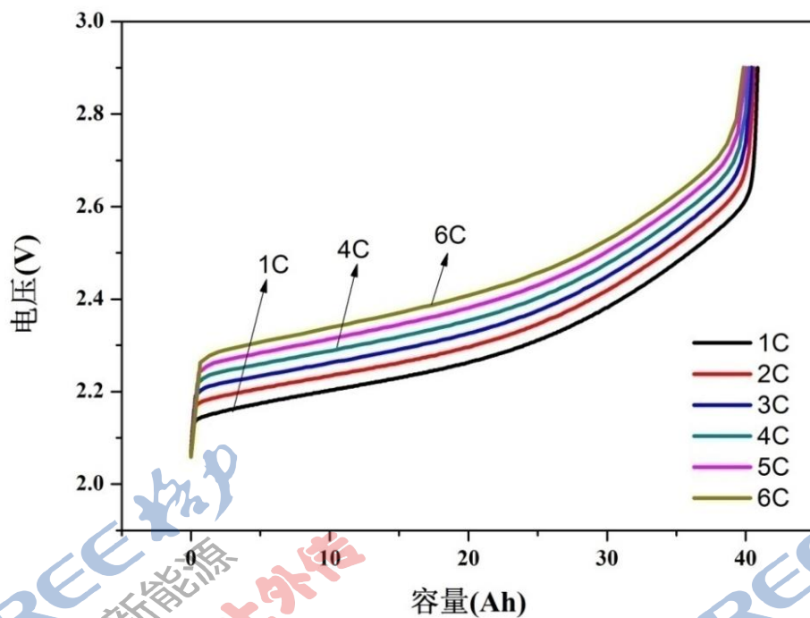
图 2 倍率充电性能曲线图 Fig.2 Rate charge performance curve
